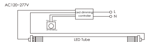
Dimming Wire Diagrams
