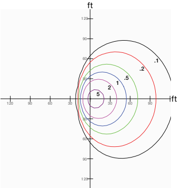
140W luminaire, mounted at 30' height, tilted 45°
