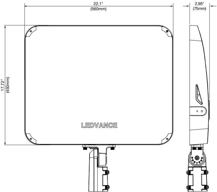
FLOOD LIGHT WITH SLIP FITTER-470W
