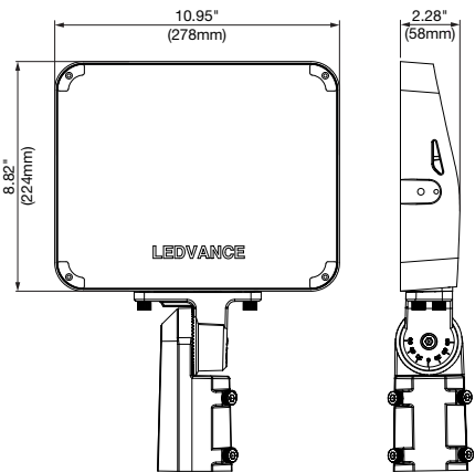
FLOOD LIGHT WITH SLIP FITTER-140W
